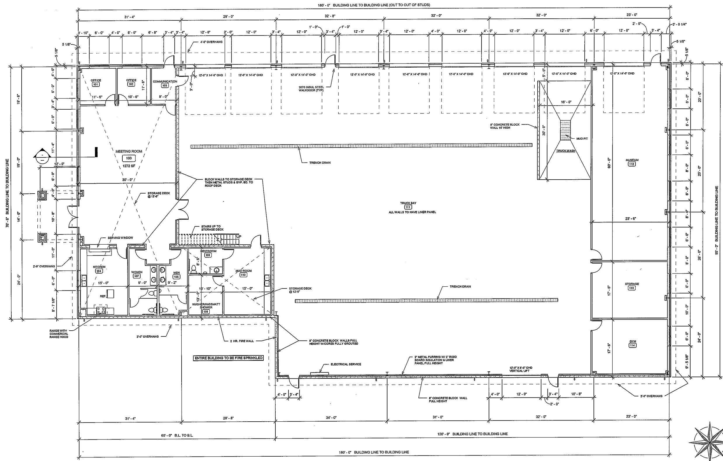
FLOOR PLAN 1/8" = 1'-0"
